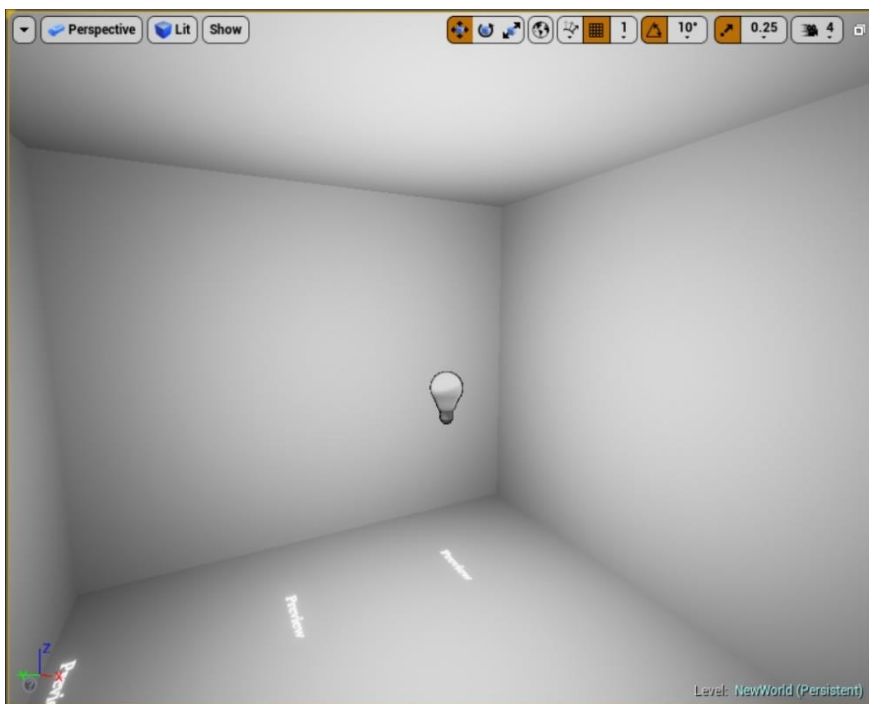
Slika 4.40. Point light.
