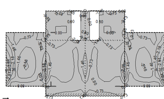
Okvir: H_2 Aa - g.zona - Pravac 1 - max Aa1,g= -4.36 cm 2 /m
