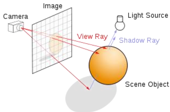
Slika 14: Ray tracing
