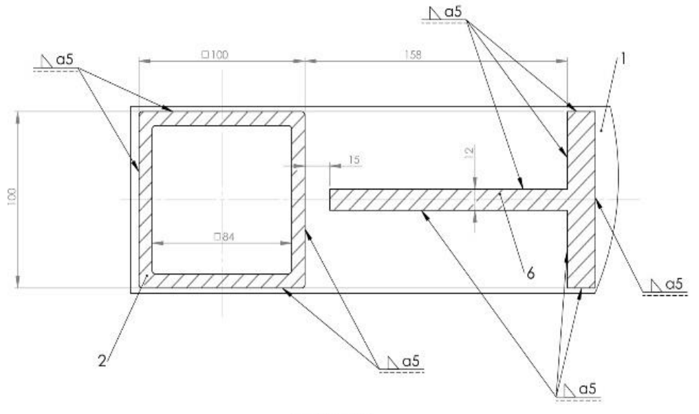
DETAIL W SCALE 1 : 2
