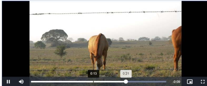
Slika 7.1 Video.js player
