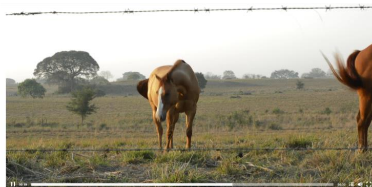
Slika 7.2 MediaElement.js player
