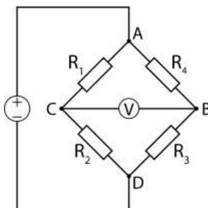
Slika 5.7 Wheatstone-ov most
