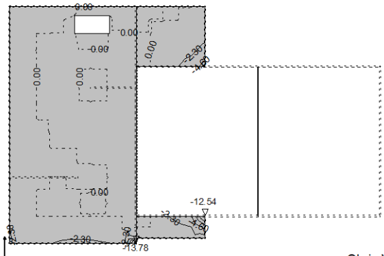
Okvir: V_1 Aa - g.zona - Pramac 2 - max Aa2,g= -13.78 cm 2 /m
