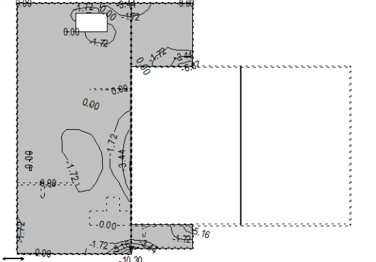
Okvir: V_1 Aa - g.zona - Pramac 1 - max Aa1,g= -10.30 cm 2 /m
