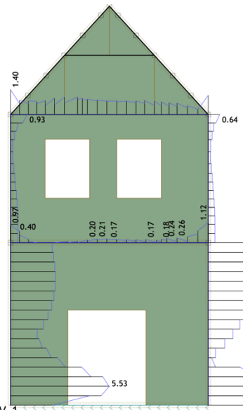
Okvir: V_1 Armatura u gredama: max \Sigma A_a = 5.53 \text{ cm}^2
