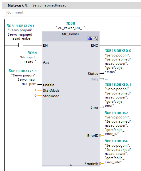
Slika 7.4.6 network 4 power
