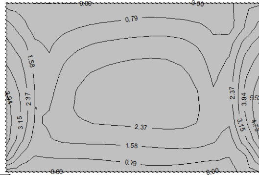
Aa - d.zona - Pravac 1 - max Aa1,d= 5.52 cm 2 /m
