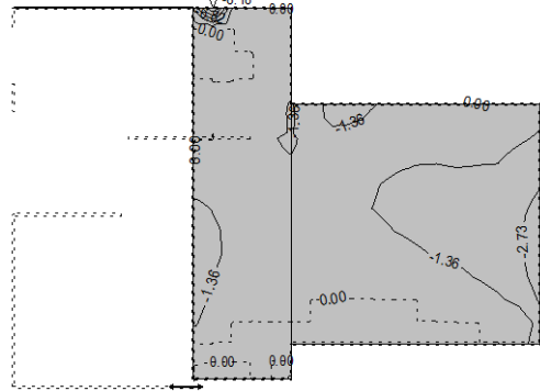
Okvir: V_5 Aa - g.zona - Pramac 1 - max Aa 1,g = -8.18 cm 2 /m
