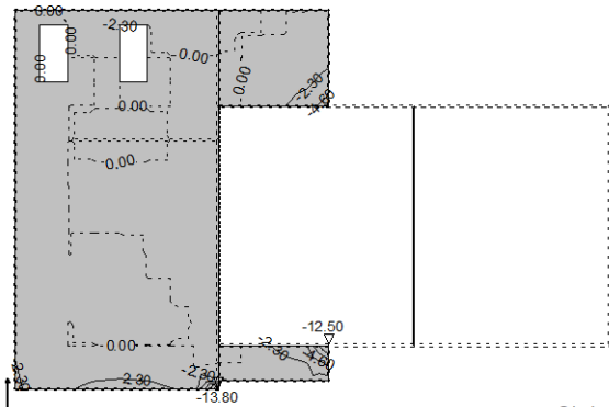
Okvir: V_2 Aa - g.zona - Pramac 2 - max Aa 2,g = -13.80 cm 2 /m
