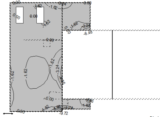
Okvir: V_2 Aa - g.zona - Pramac 1 - max Aa 1,g = -9.72 cm 2 /m
