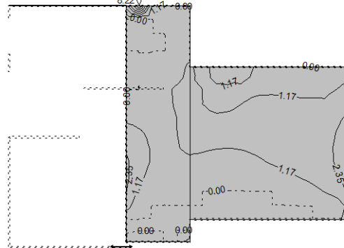
Okvir: V_5 Aa - d.zona - Pramac 1 - max Aa 1,d = 8.22 cm 2 /m
