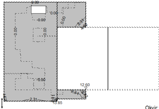
Okvir: V_1 Aa - d.zona - Pramac 2 - max Aa 2,d = 13.85 cm 2 /m
