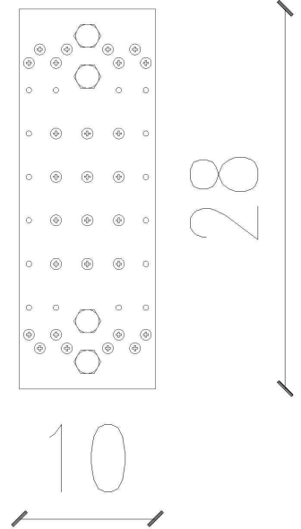
RASPORED VIJAKA 1:5
