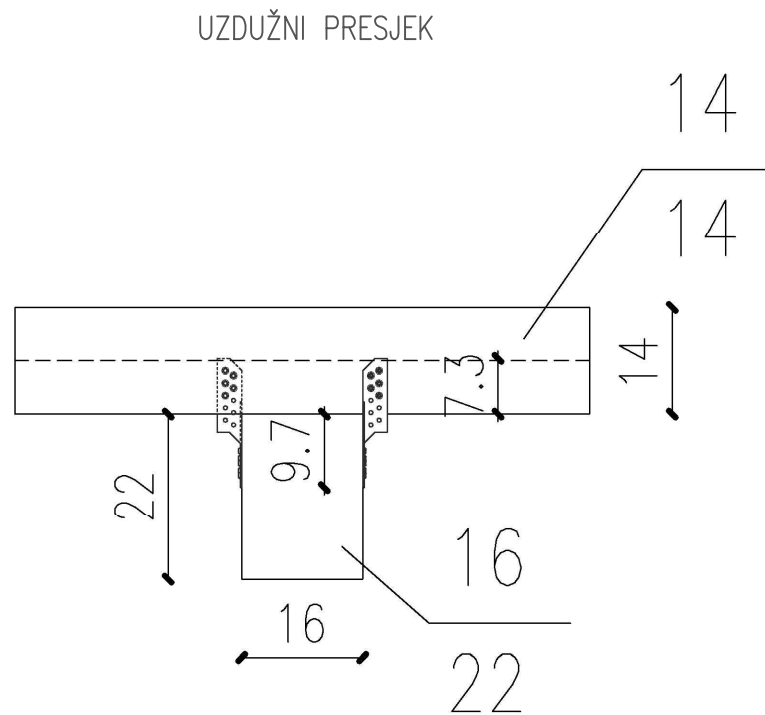
RASPORED VIJAKA 1:5
