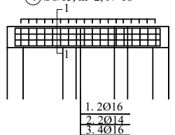
G208 ④ Ø8/15, m=2, N=18
