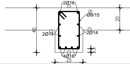
ISKAZ REBRASTE ARMATURE - ČELIK B500B
