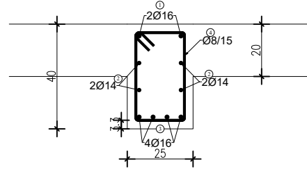
ISKAZ REBRASTE ARMATURE - ČELIK B500B
