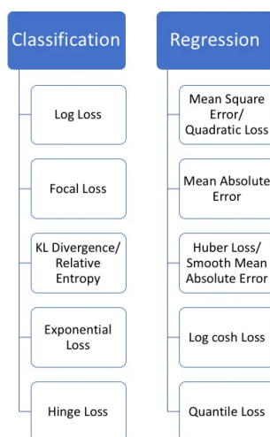
Slika 7-1 Podjela funkcije gubitka (Preuzeto 10.7.2024. s https://heartbeat.comet.ml/5-regression-loss-functions-all-machine-learners-should-know-4fb140e9d4b0 )
